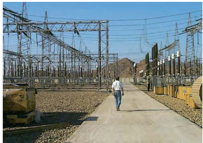
Fig. 3.1-16: Central/center tower arrangement, 220 kV, Egypt
