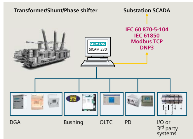
Fig. 5.13-3: System platform
