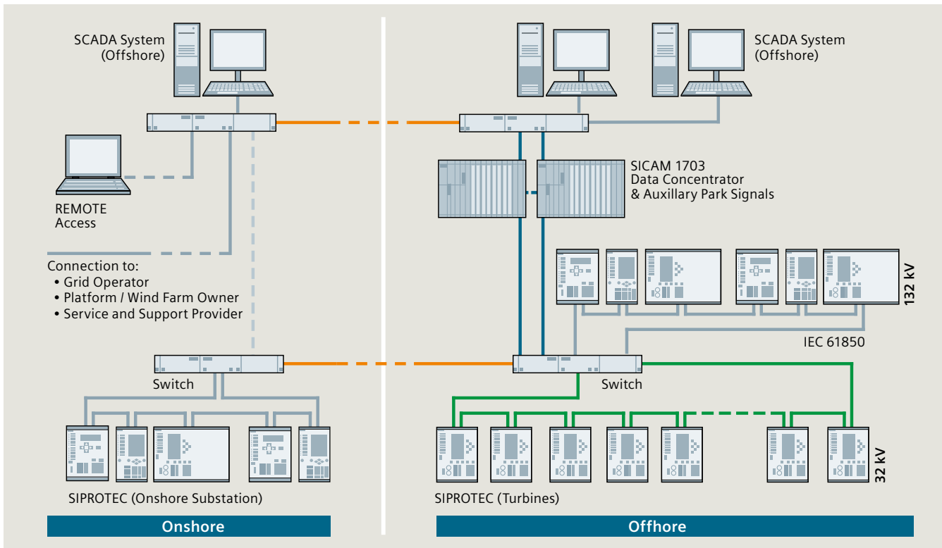
Fig. 6.6-26: SCADA system with onshore and offshore part
