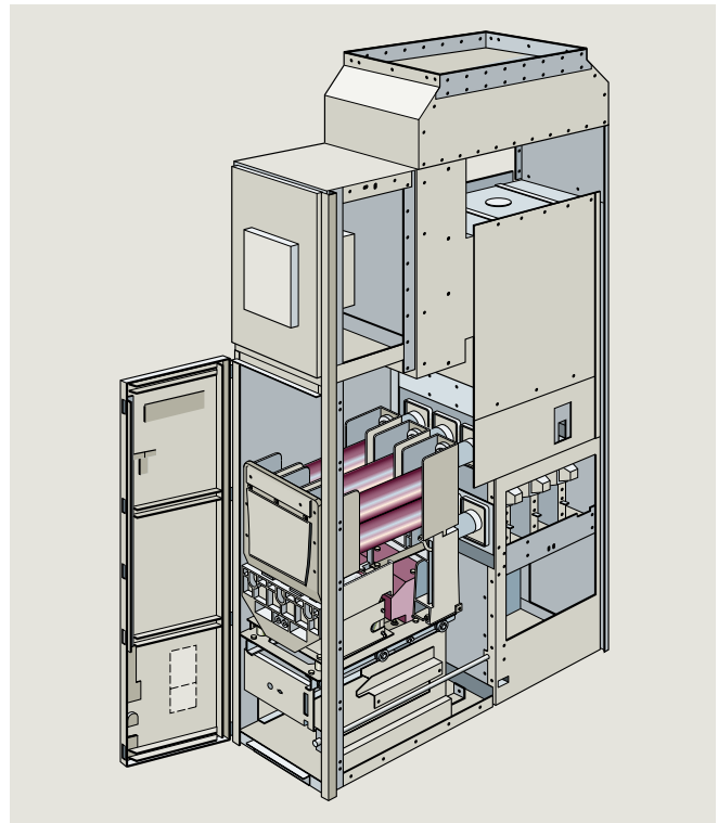
Fig. 4.3-14: Installation of the contactor-fuse combination in the contactor panel
