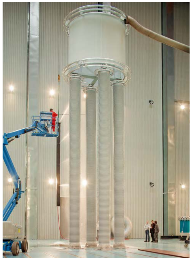
Fig. 4.2-36: Pole bus smoothing reactor for UHVDC Agra (BIL 1,300 kV; 2,680 A; 75 mH) – tests at HSP Cologne
