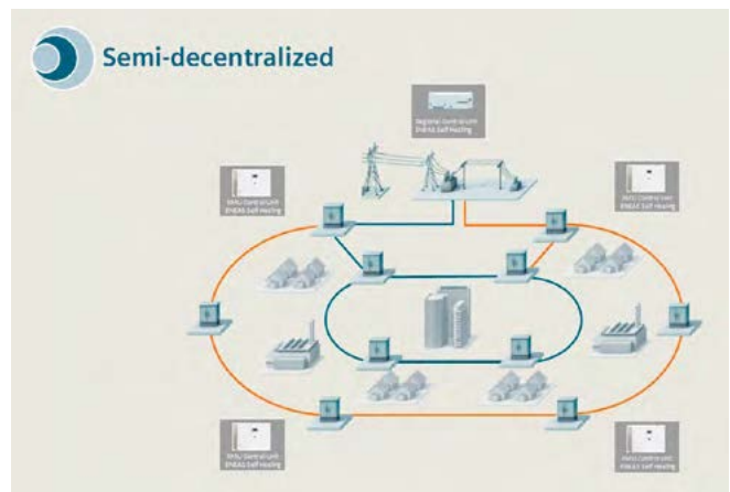
Fig. 6.6-16: Semi-decentralized architecture
