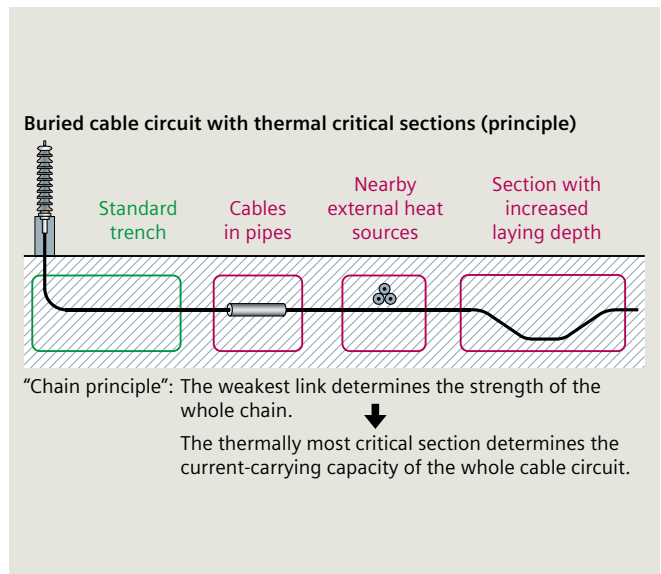
Fig. 2.2-60: Different laying arrangements in ground
