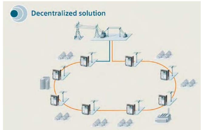
Fig. 6.6-15: Decentralized architecture
