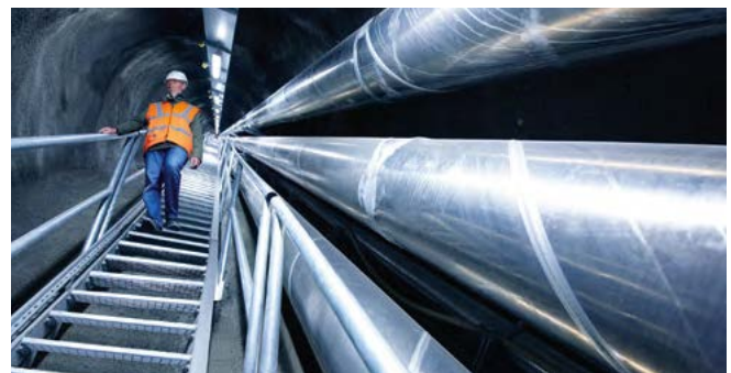
Fig. 2.2-49: GIL laid in shaft with 42° gradient (Limberg, Kaprun, Austria)
