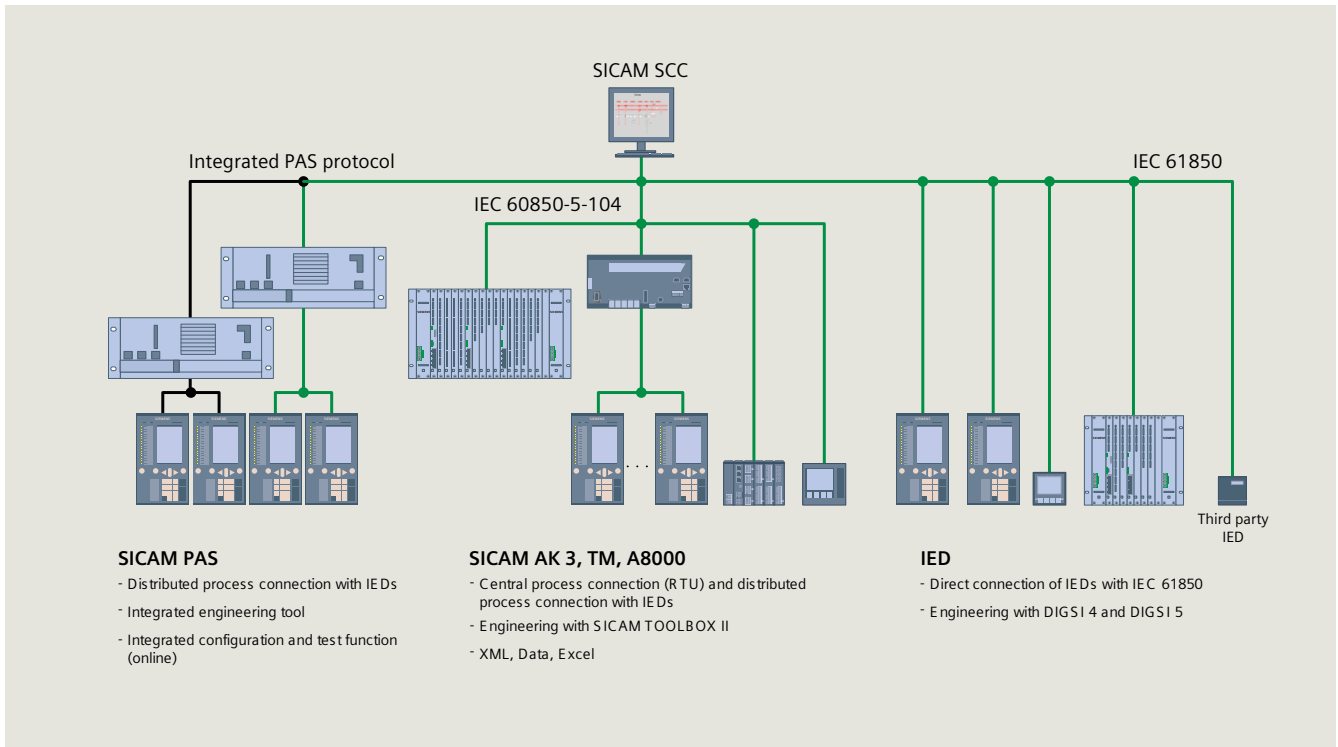
Fig. 6.3-8: Flexible configuration
