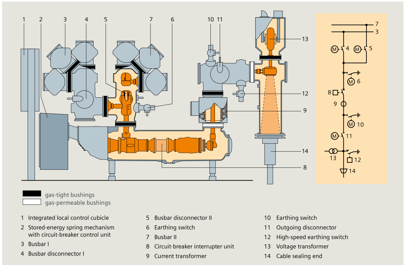
Fig. 3.1-38: 8DQ1 switchgear bay up to 420 kV
