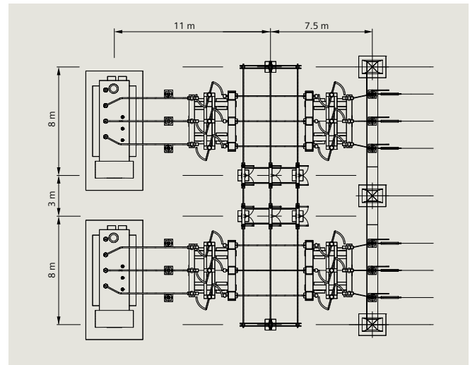
Fig. 3.1-24: SIMOBREAKER (schematic)
