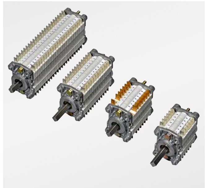
Fig. 4.3-15: Auxiliary switch 3SV9
