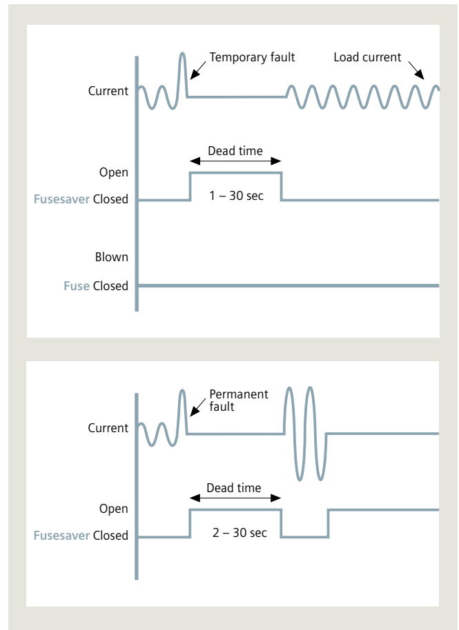
Fig 4.3-12: Modes of operation of the Fusesaver
