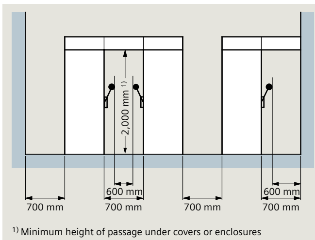
Fig. 3.3-12: Reduced gangway widths within the area of open doors
