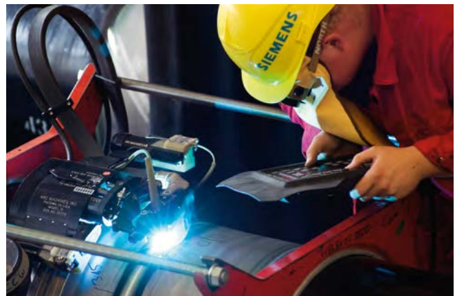
Fig. 2.2-44: Orbital welding of GIL pipes
