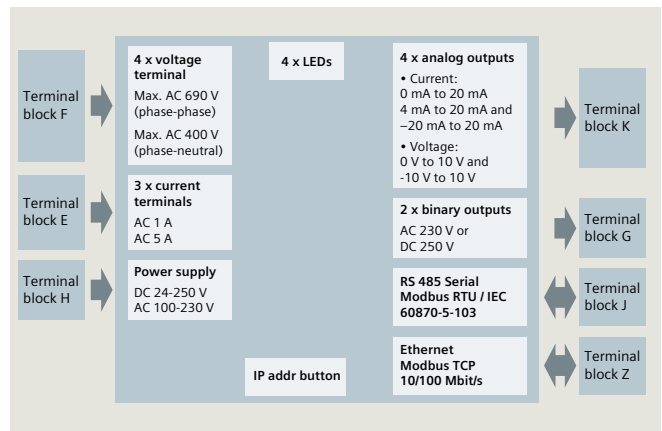
Fig. 6.4-14: Block diagram SICAM T 7KG9661
