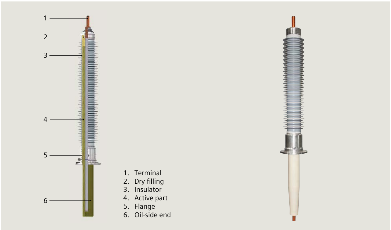
Fig. 4.2-42: Transformer bushing – resin-impregnated paper (RIP) design – sectional view
