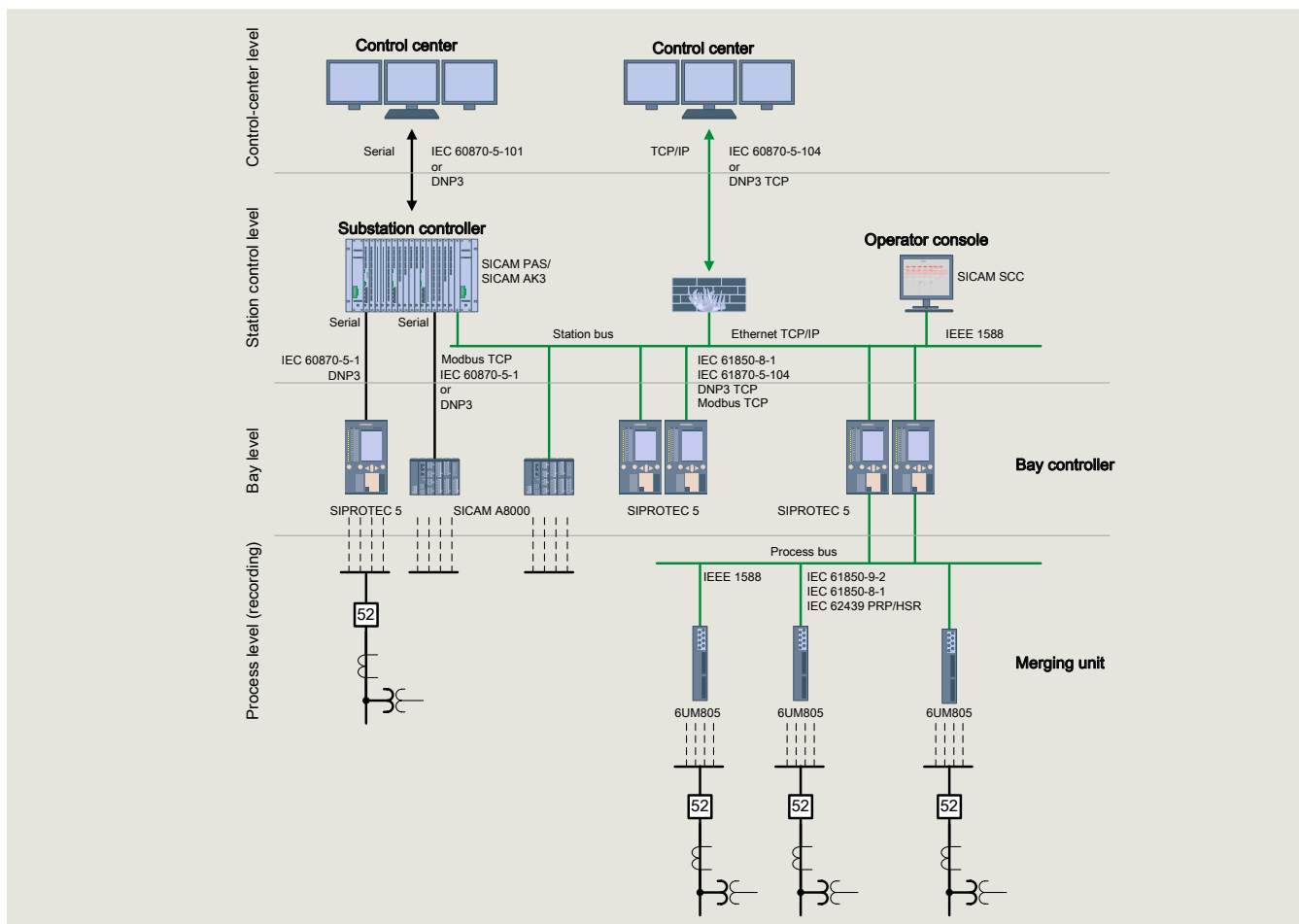
Fig. 6.5-1: Example of protection and substation communication
