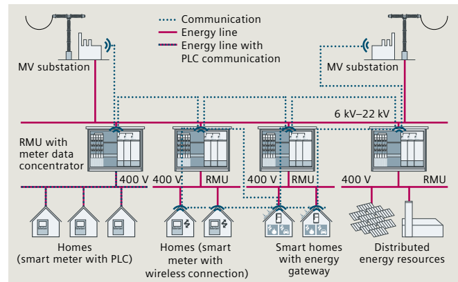
Fig. 8.3-5: Wireless mesh network
