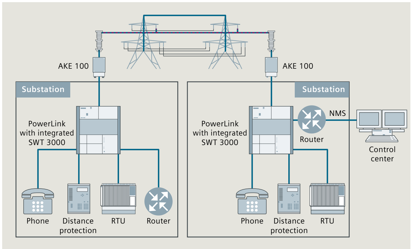
Fig. 8.1-4: PowerLink high-voltage line communication
