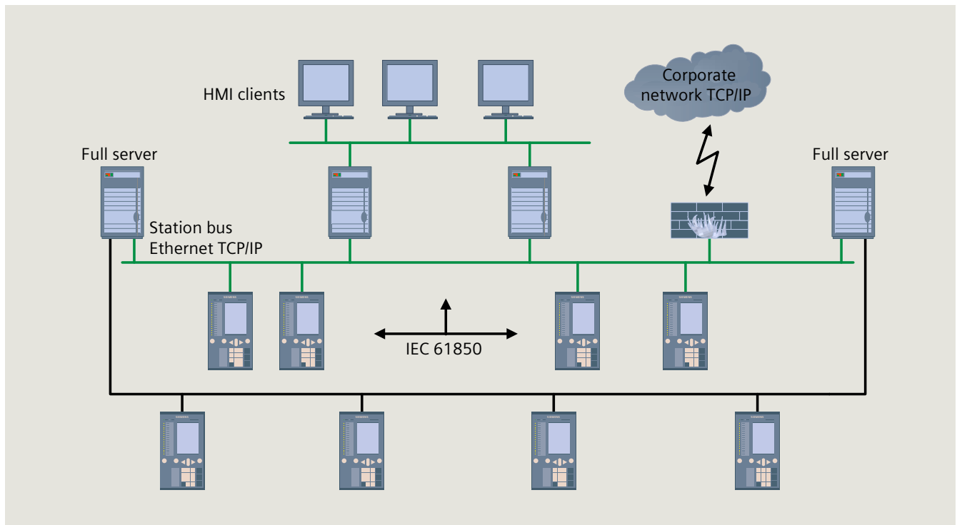
Fig. 6.3-6: Typical redundant configuration: Full server and HMI server are based on a redundant structure to boost availability
