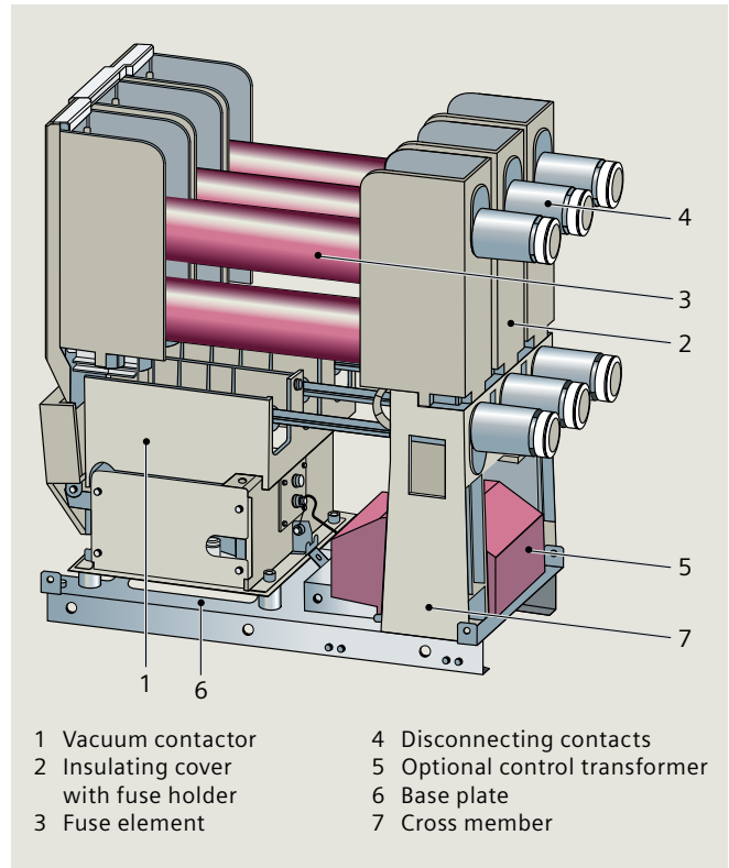
Fig. 4.3-13: Construction of the contactor-fuse combination 3TL6
