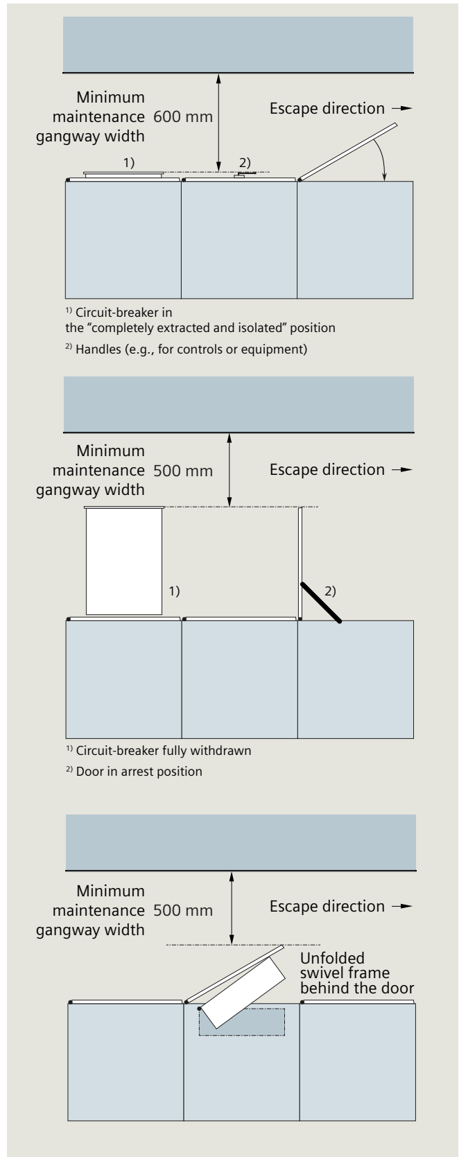
Fig. 3.3-13: Minimum widths of maintenance gangways in accordance with IEC 60364-7-729 (VDE 0100-729)
