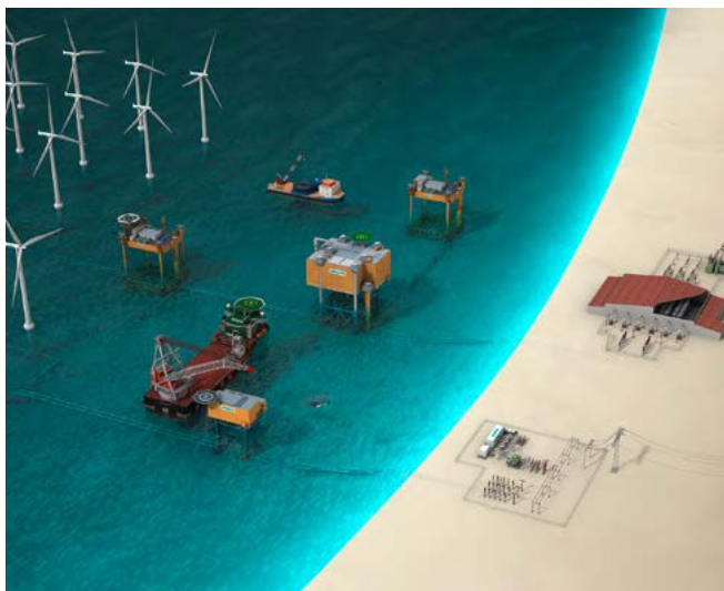
Fig. 2.2-27: A comprehensive overview for both AC and DC offshore wind farm grid connections
