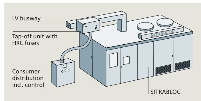
Fig. 3.2-41: Location sketch
